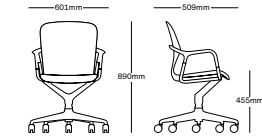
Chair with five-star base
